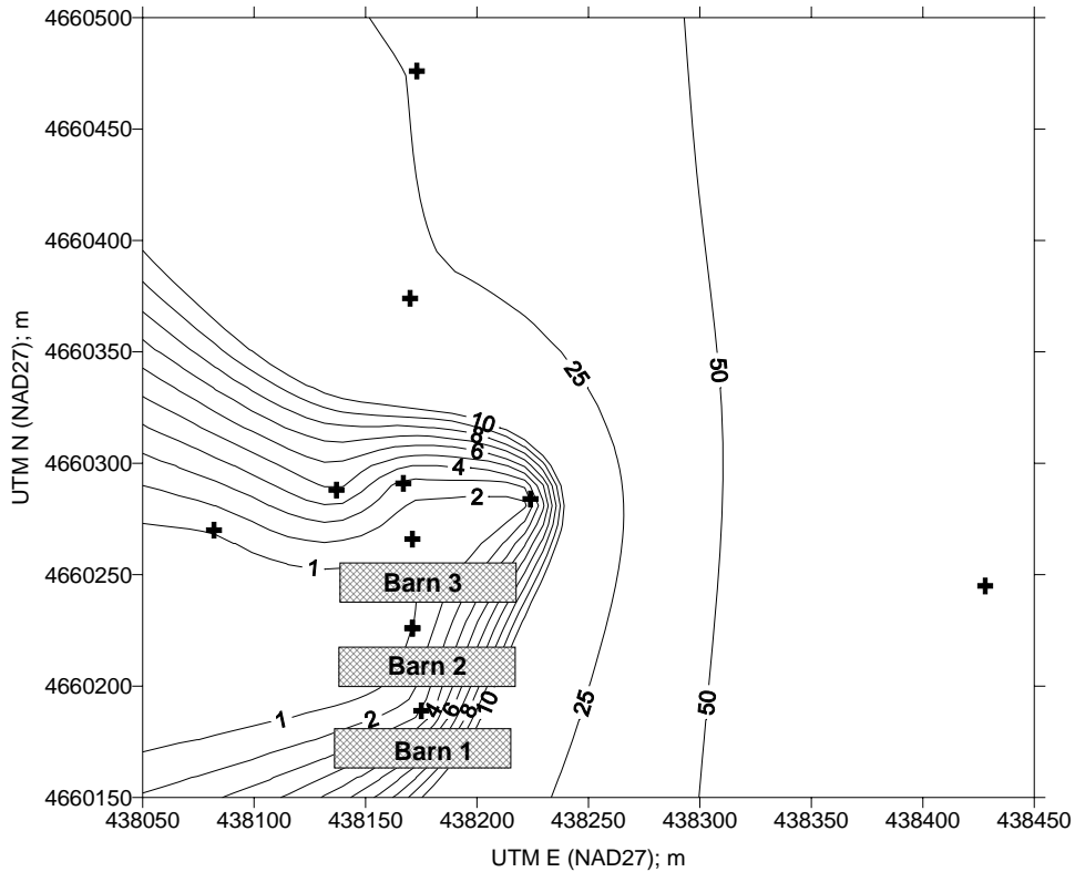
Figure 2. Isoleptic map of the overall averaged ratio of the observed NH 3 concentrations to the modeled NH 3 concentrations.
